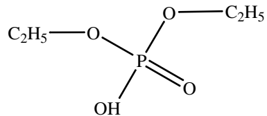
diethyl acid phosphate
